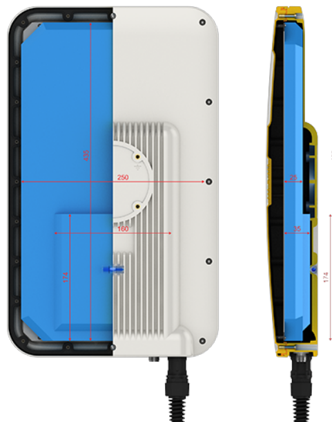
Inner dimensions WiBOX Extra Large Slim
