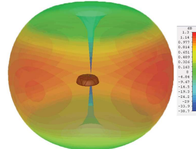
Typical 3D Pattern (2100MHz)
