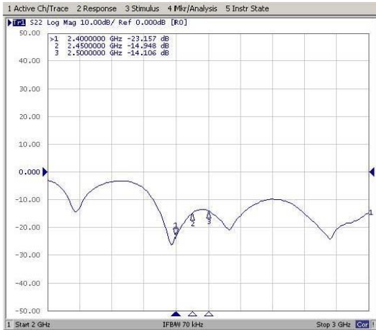
Return Loss
