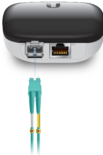
Connect a fiber optic cable. (UFiber ODN cable, model UOC-5 shown)
