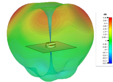
Typical 3D Pattern - 4G/5G Elements 1800MHz
