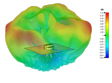
Typical 3D Pattern - 4G/5G Elements 3600MHz
