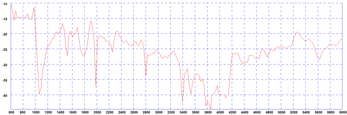
Typical Isolation - 4G/5G Elements*
