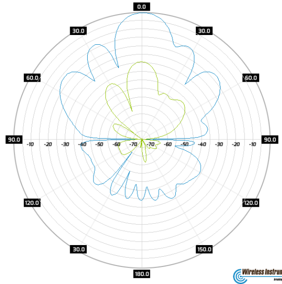
Radiation Pattern Port 2 Pol 2
