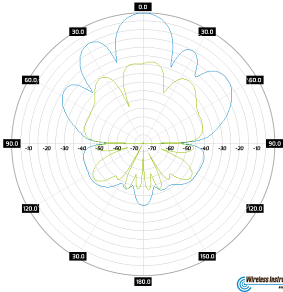
Radiation Pattern Port 2 Pol 1
