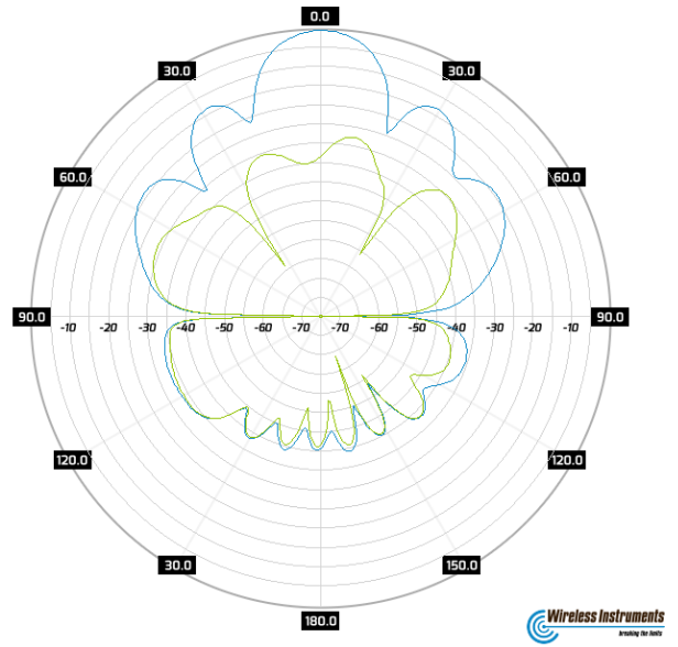
Radiation Pattern Port 2 Pol 2
