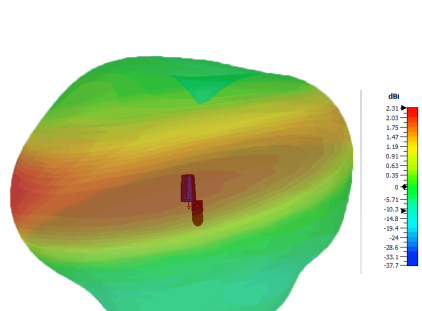
3D Plot (2600 MHz)
